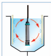
Measurement of activated sludge density
