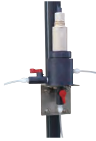
probe-type Detector W/Flow type holder NCD-3P/10P-LQ +LQ-FL-45
